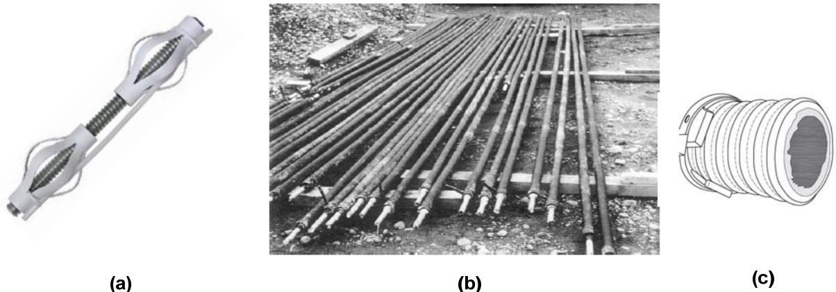
Gambar 48 – Material pelengkap: a) centralizer (FHWA-NHI-14-007), b) nail bar dibungkus corrugated sheath pada soil nailing permanen (FHWA0-IF-03-017), c) corrugated sheath (BS 8006-2, 2011)
